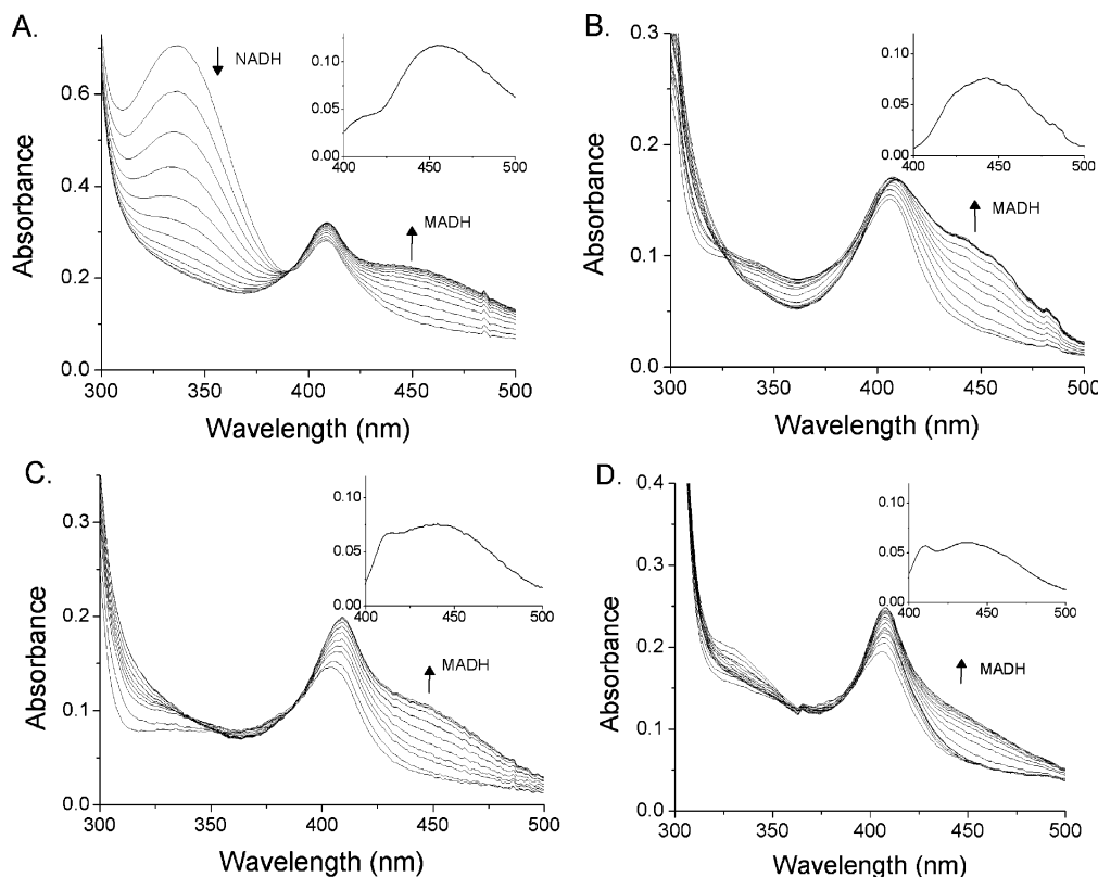
FIGURE 2: Spectrophotometric assay of TTQ biosynthesis. Each reaction mixture contained 0.5 \mu\text{M} MauG and 10 \mu\text{M} MADH biosynthetic intermediate in 10 \text{ mM} potassium phosphate at pH 7.5. Reactions were performed under aerobic conditions and initiated by the addition of 100 \mu\text{M} NADH (A), 250 \mu\text{M} DTT (B), 250 \mu\text{M} GSH (C), or 500 \mu\text{M} ascorbic acid (D). The arrows indicate the direction of the spectral changes. The spectra were recorded every 2 min for 22 min in A and B, every 10 min for 110 min in C, and every 10 min for 150 min in D. The difference spectrum of the final minus the initial spectrum in the region of interest is shown in each inset. In each spectrum, the absorption peak centered on 406\text{--}416 \text{ nm} is due to the MauG present in each sample.
